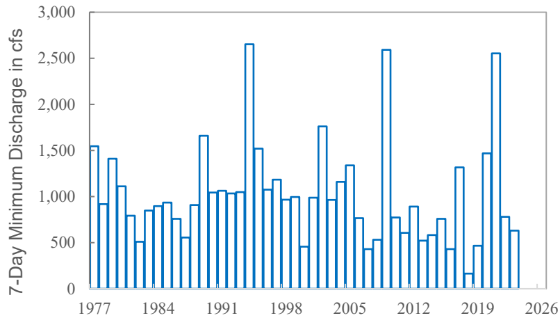
Plot of 7-Day Minimum Flows
