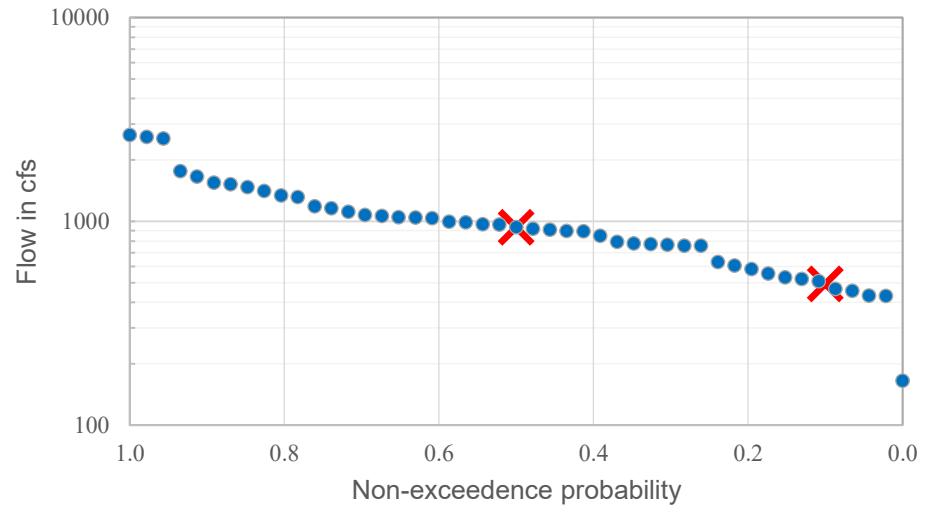
Low-Flow (7-Day Minimum) Frequency Curve
